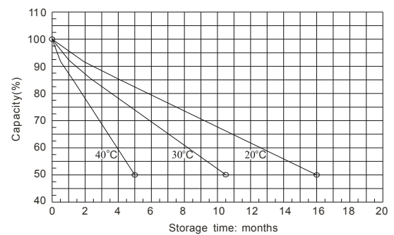
Self-discharge characteristic
