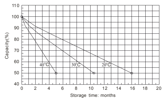
Self-discharge characteristic
